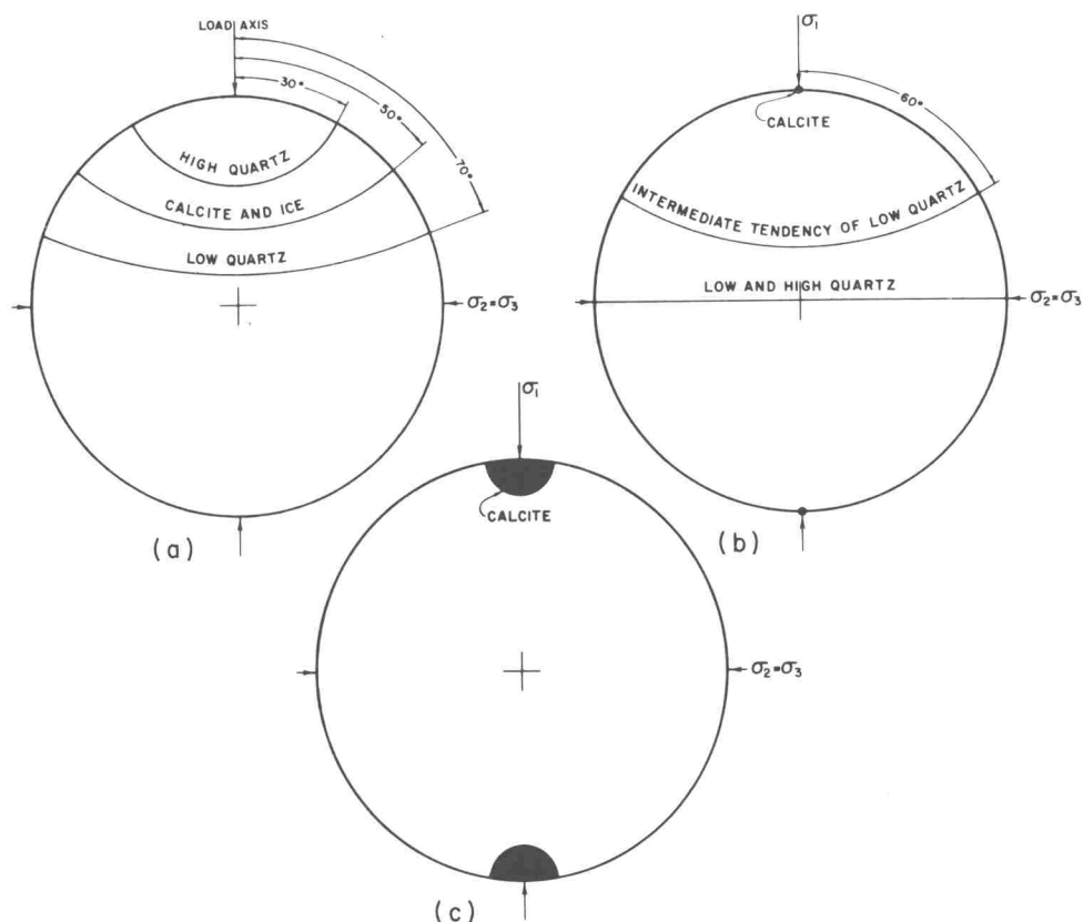
Fig. 47—Stereograms showing the predicted (a and b) and the experimentally determined (c) orientations of c_v in minerals recrystallized under a uniaxial state of stress (stereographic projection). (a) Orientations of c_v predicted by MacDonald (165) and calculated by Brace (Ref. 169, Fig. 4) for calcite, ice, high and low quartz. (b) Orientations of quartz and calcite c_v predicted by Kamb (167) for recrystallization in the presence of a fluid phase. (c) Orientation of calcite c_v produced in experiments as a result of syntectonic, dry recrystallization.
